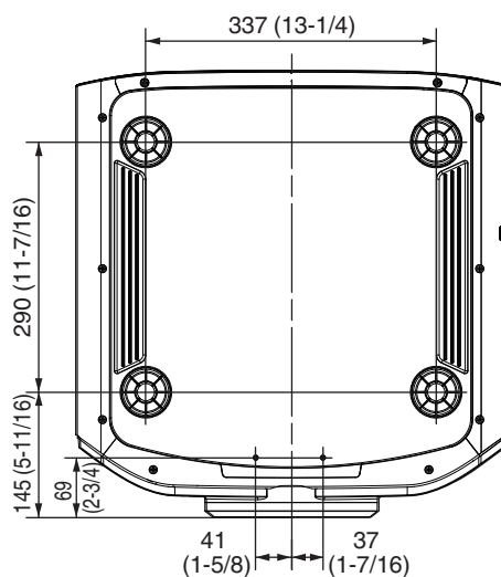
Bottom Surface
